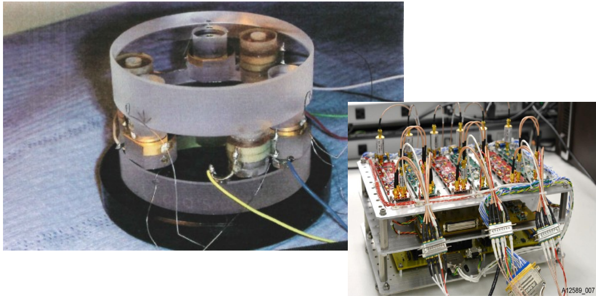
Figure 7: Ball Aerospace Sensor and Control Demonstration Article
