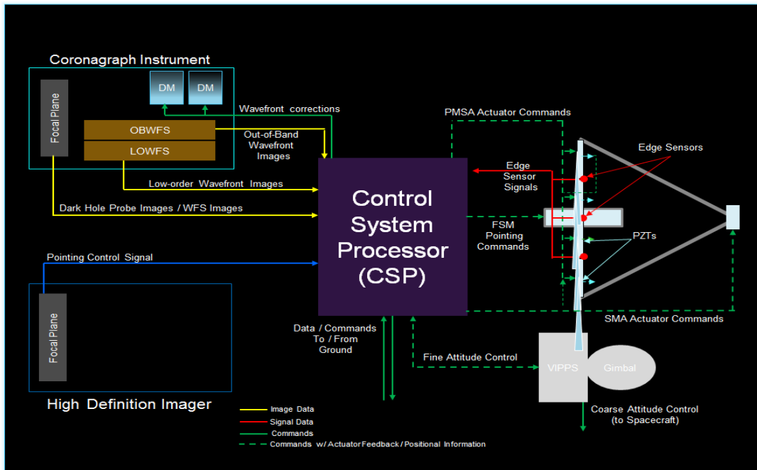
Figure 4: Control Architecture
