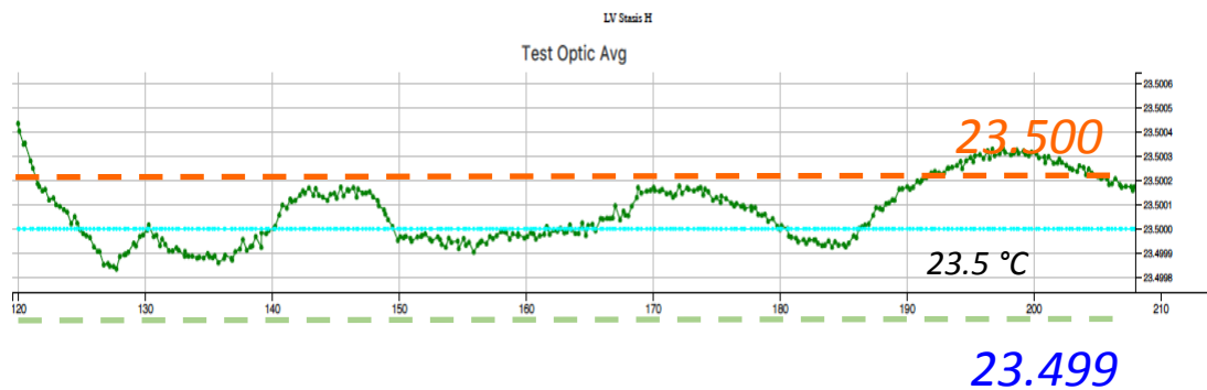
Figure 10: Surrogate Test Article that Demonstrated 1 Milli-Kelvin Control
