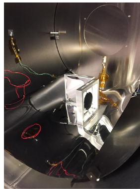
Figure 9: Surrogate Test Article that Demonstrated 1 Milli-Kelvin Control
