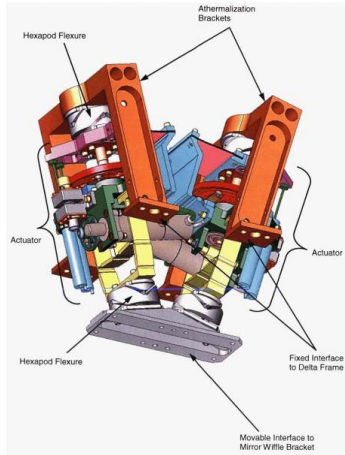
Figure 8: Heritage JWST Bipod
