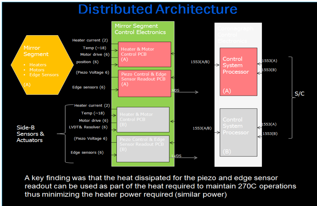
Figure 5: Distributed Control Architecture
